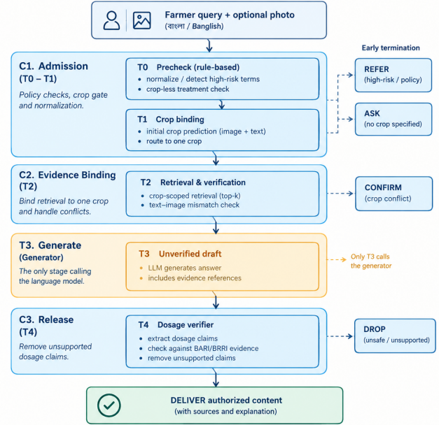
Figure 1: KrishokTech places five control stages (T0–T4) before delivery. T0 can end a request in REFER , T1 in ASK , and T2 in CONFIRM . T3 produces an unverified draft; T4 removes unsupported dosage claims before the remaining text is delivered.
